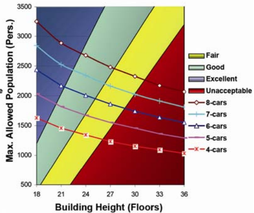
Max. Allowed Population Vs Number of Floors, HC of 17% / 5 min, 2x24 Person Rated Load, Speed = Travel / 20s
