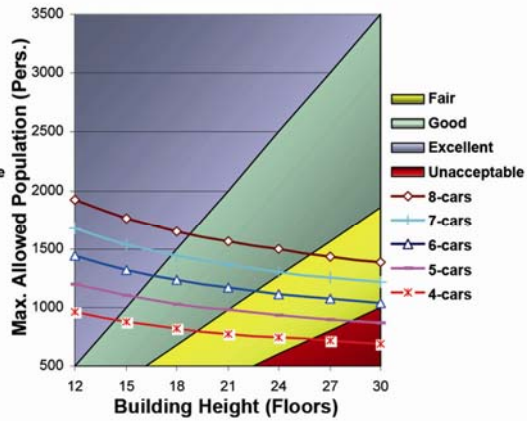
Max. Allowed Population Vs Number of Floors, HC of 13% / 5 min, 21 Person Rated Load, Speed = Travel / 20s
