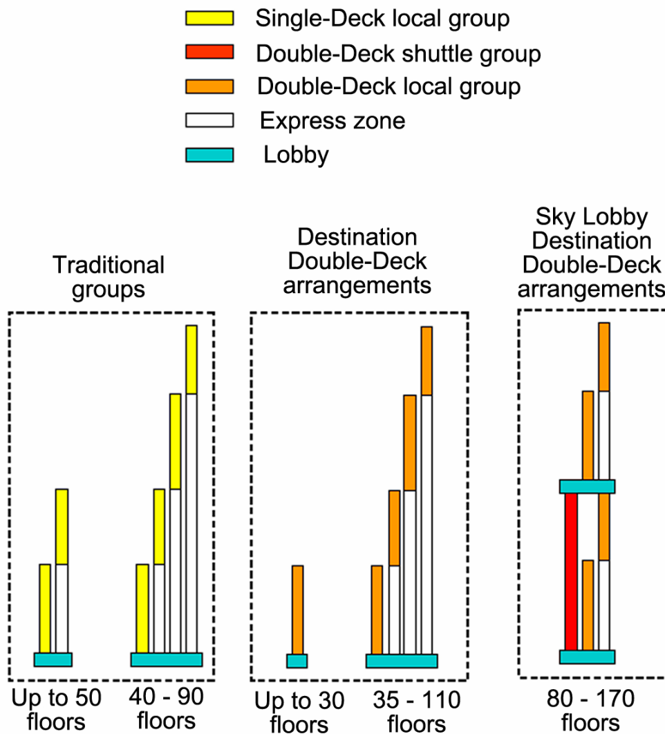
Figure 4. Building stacking diagrams with Hall Call Destination Dispatching systems (KONE Corporation).
