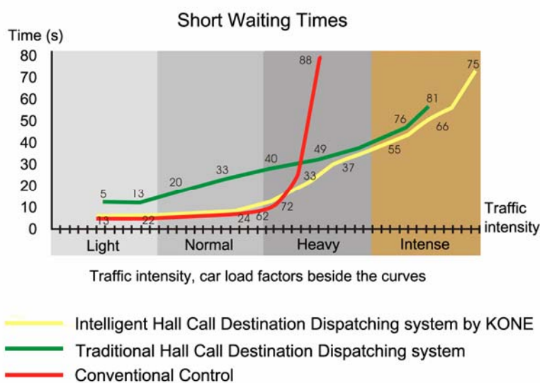
Figure 3. The Intelligent Hall Call Destination Dispatching system can provide the shortest waiting times and the maximum handling Capacity when needed (KONE Corporation).
