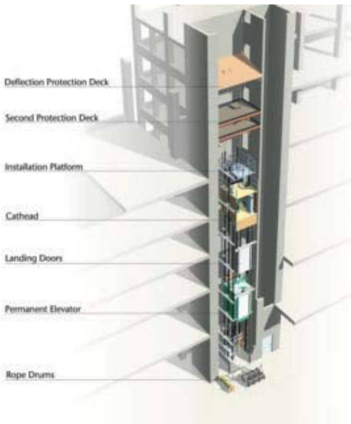
Labeled shaft diagram
