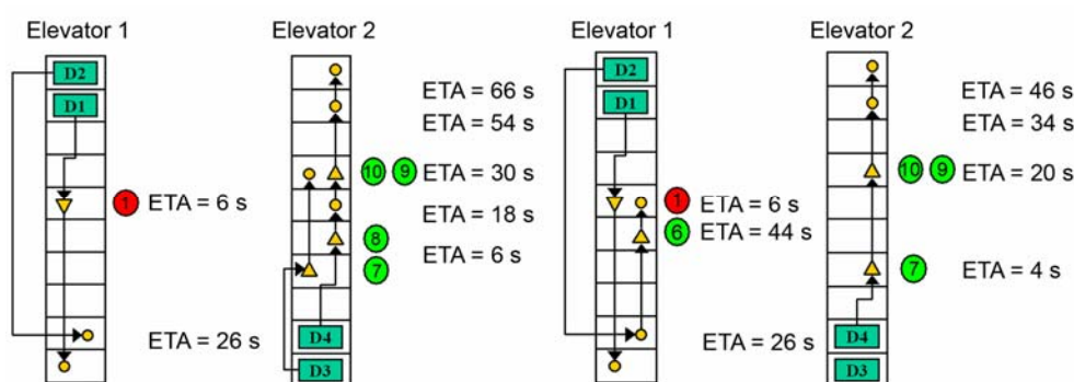
Figure 4. Double-deck elevator routing with destination calls
