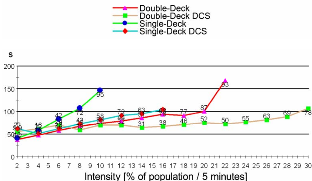
Figure 6. Simulated times to destination for different elevator arrangements
