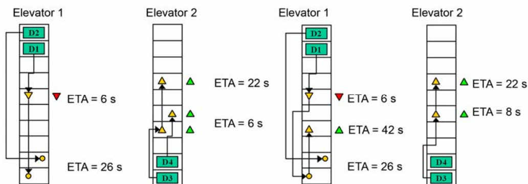
Figure 2. Double-deck elevator routing with the given solution candidates
