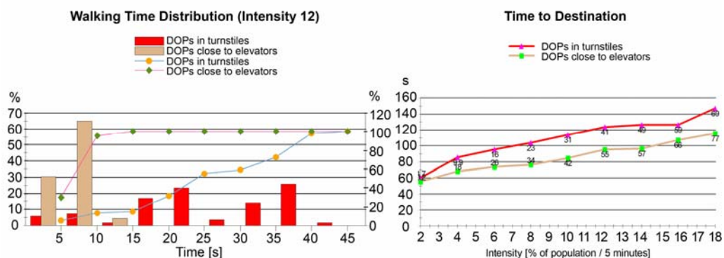
Figure 5. Walking time distribution for different floor layouts at 12% intensity and simulated times to destination
