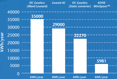
KONE MiniSpace™ energy consumption compared to previous technologies
