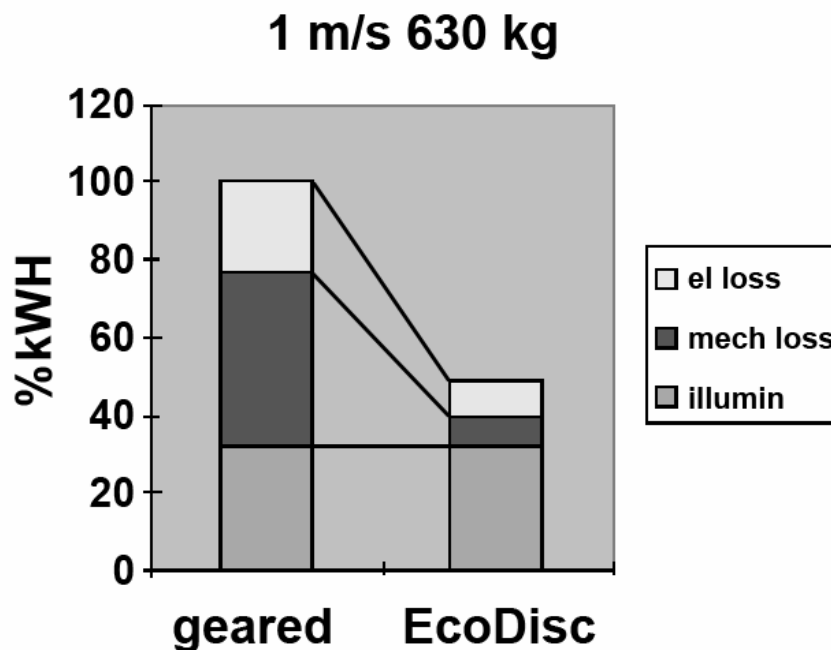
Figure 3. Energy comparison
