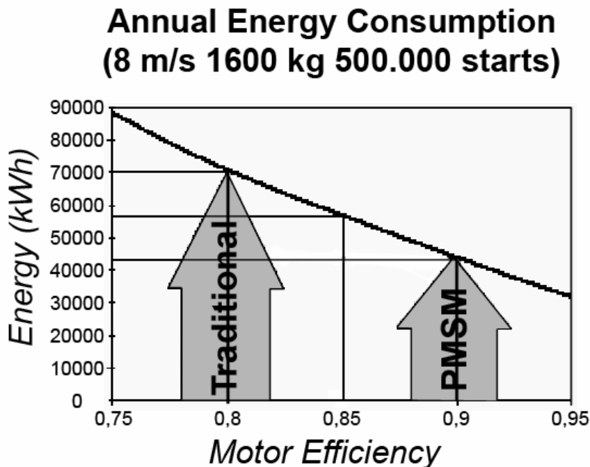
Figure 7. Energy savings with EcoDisc® PMSM motors
